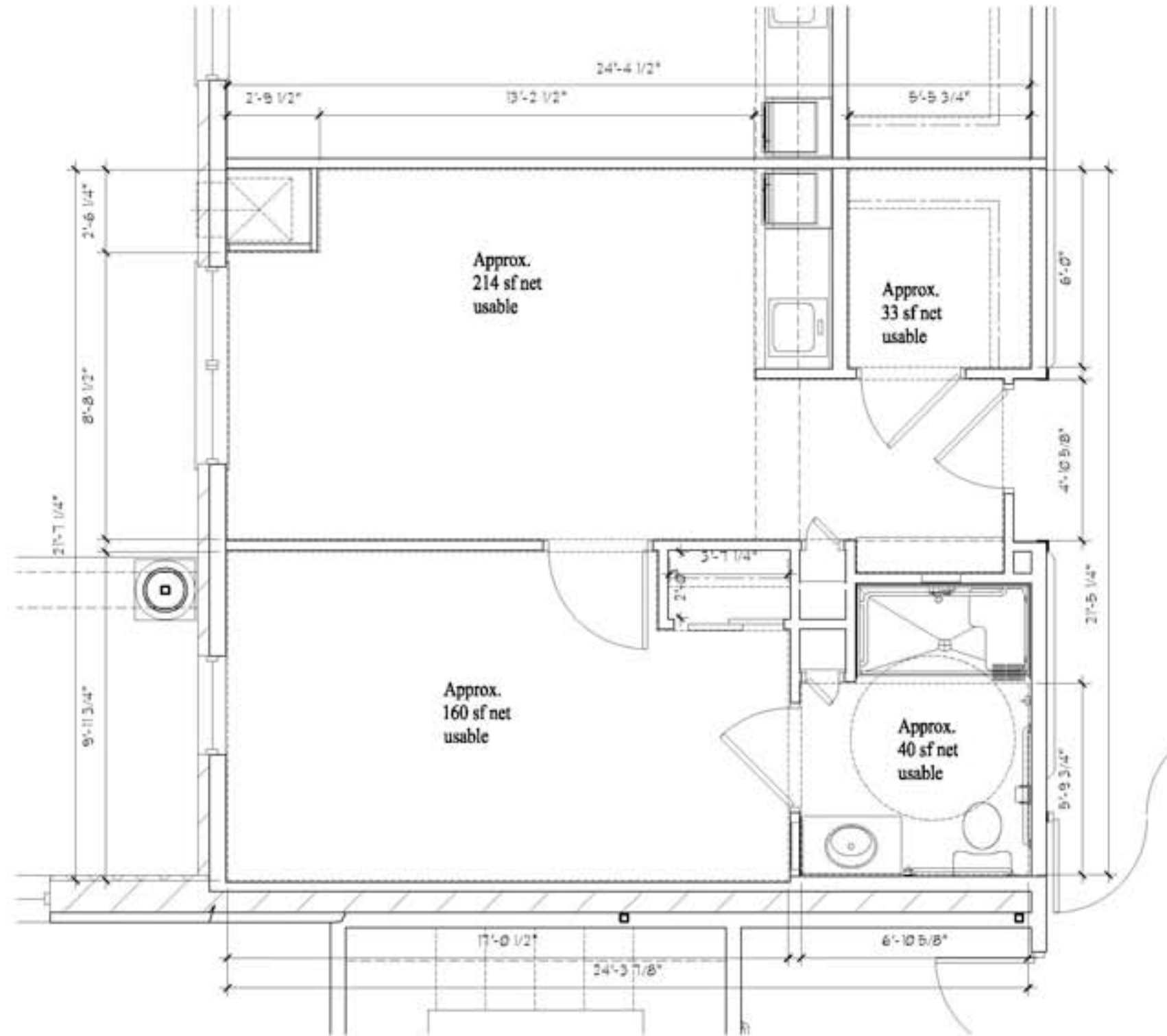
Assisted Living Unit Type A \frac{1}{4}'' = 1'-0'' 535 sf gross
