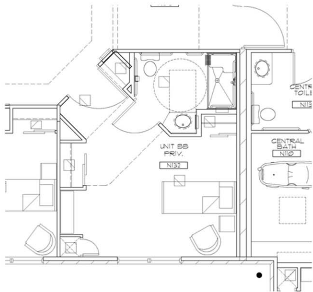
Nursing Unit Type BB- Private \frac{1}{4}''=1'-0'' 315sf
